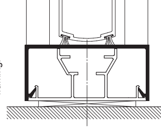
Pivot door framing.
